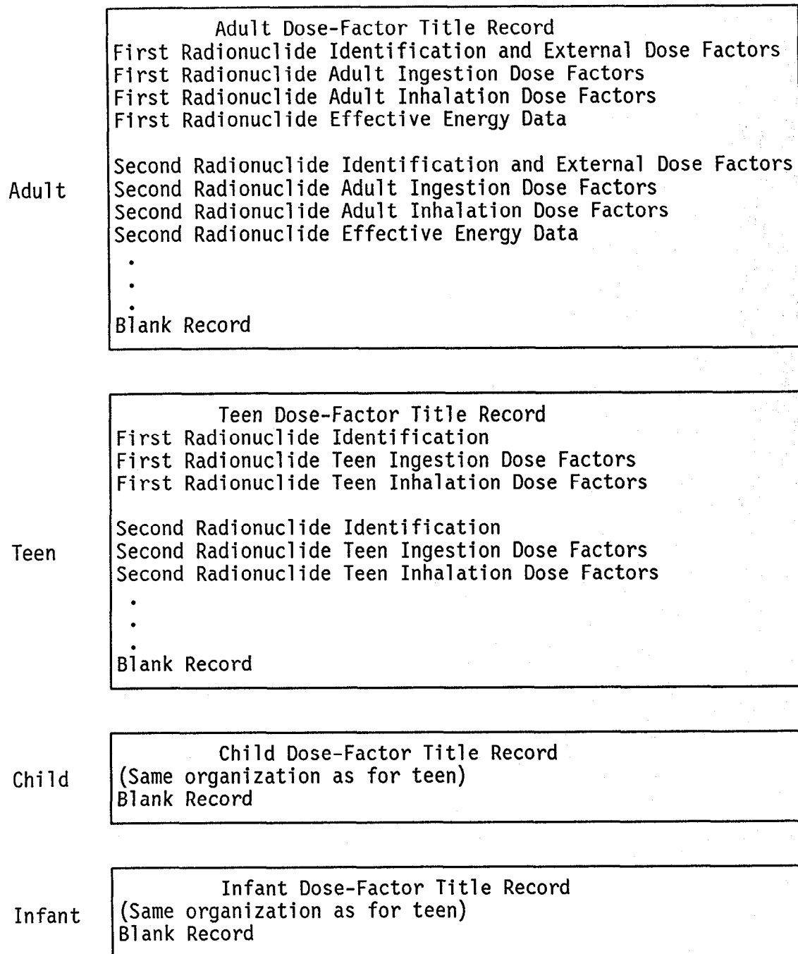
FIGURE 4.8. Dose-Factor Library Structure
