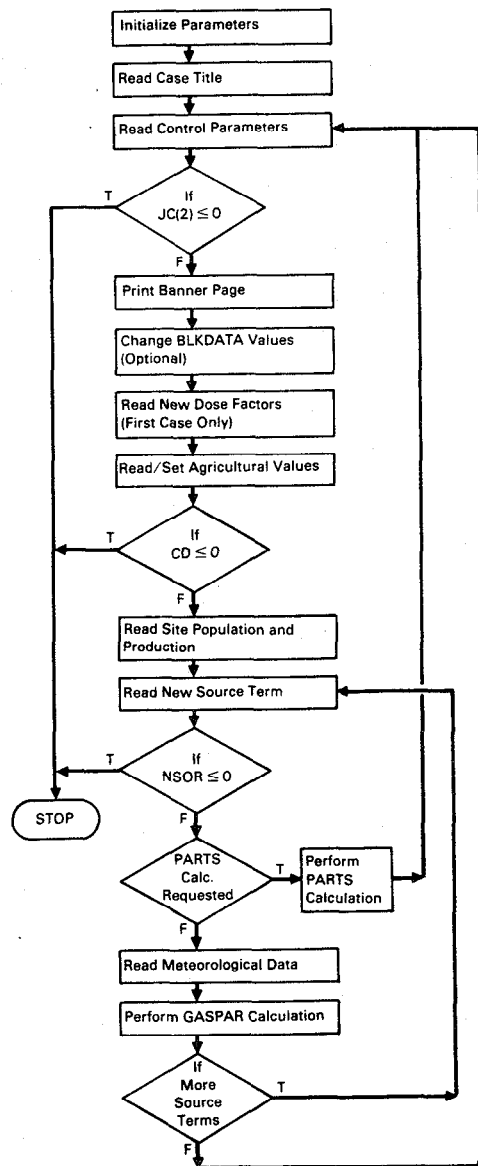
FIGURE 4.2. Main Program Structure and Control Logic
